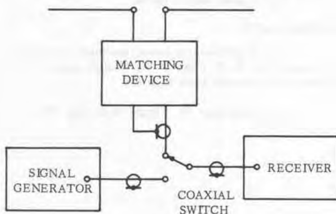
FIGURE 1. EQUIPMENT SETUP
