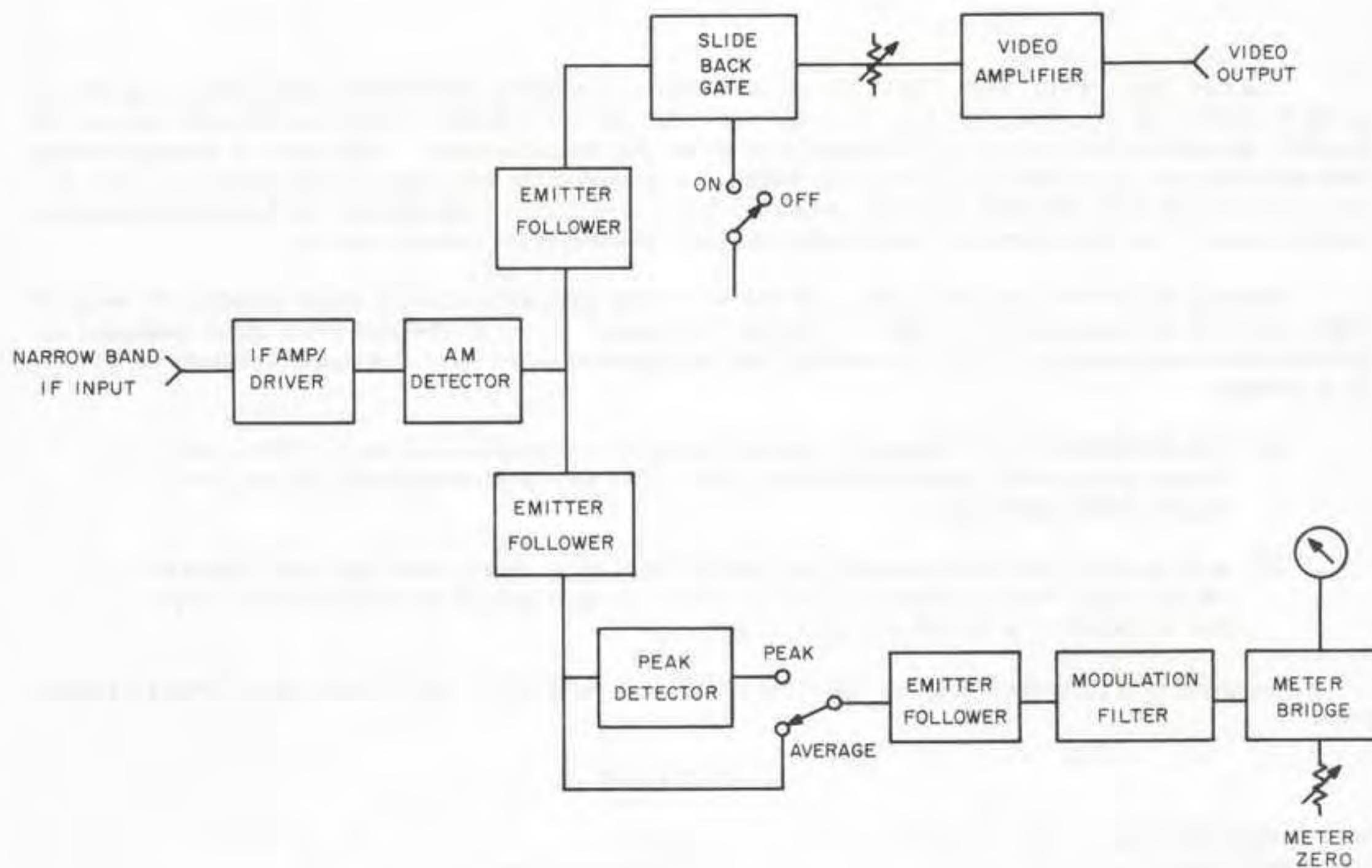
Type MP-101 Meter Panel, Functional Block Diagram
