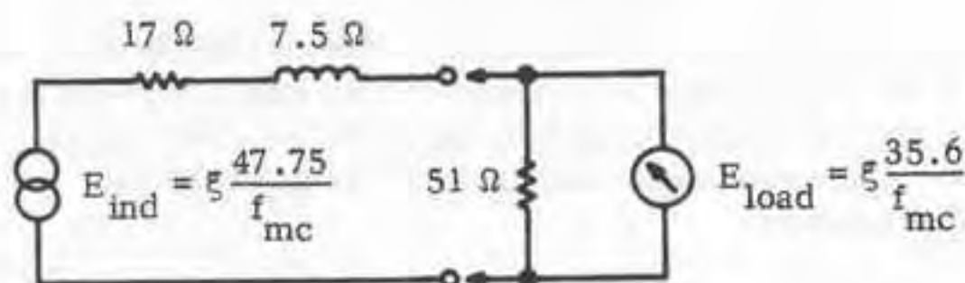
FIGURE 3. EQUIVALENT CIRCUIT, IMPEDANCE TRANSFORMED
