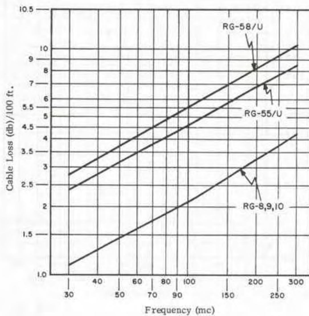
FIGURE 4. CABLE LOSS
